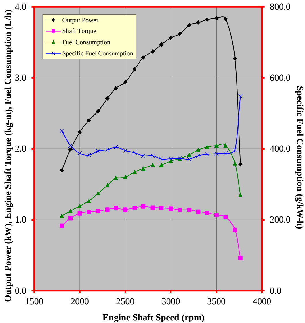
Figure 3. Performance characteristic curves of the HONDA GX200H QM gasoline engine
