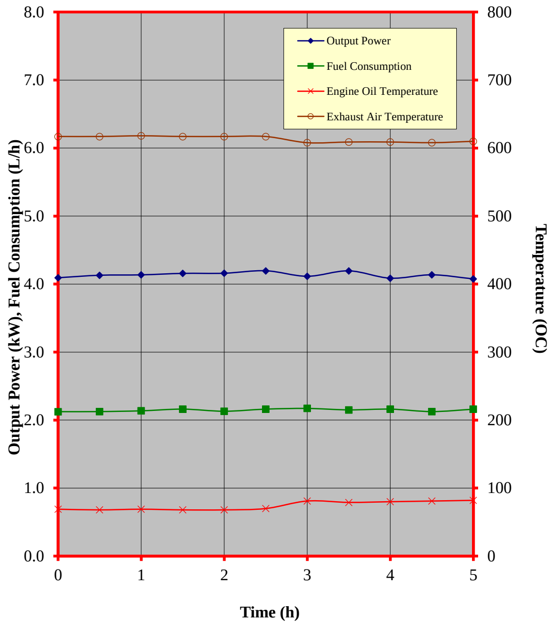
Figure 4. Performance characteristic curves during the continuous running test of the HONDA GX200H QM gasoline engine
