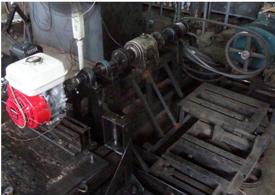
Figure 2. Test set-up of the HONDA GX200H QM Gasoline Engine
